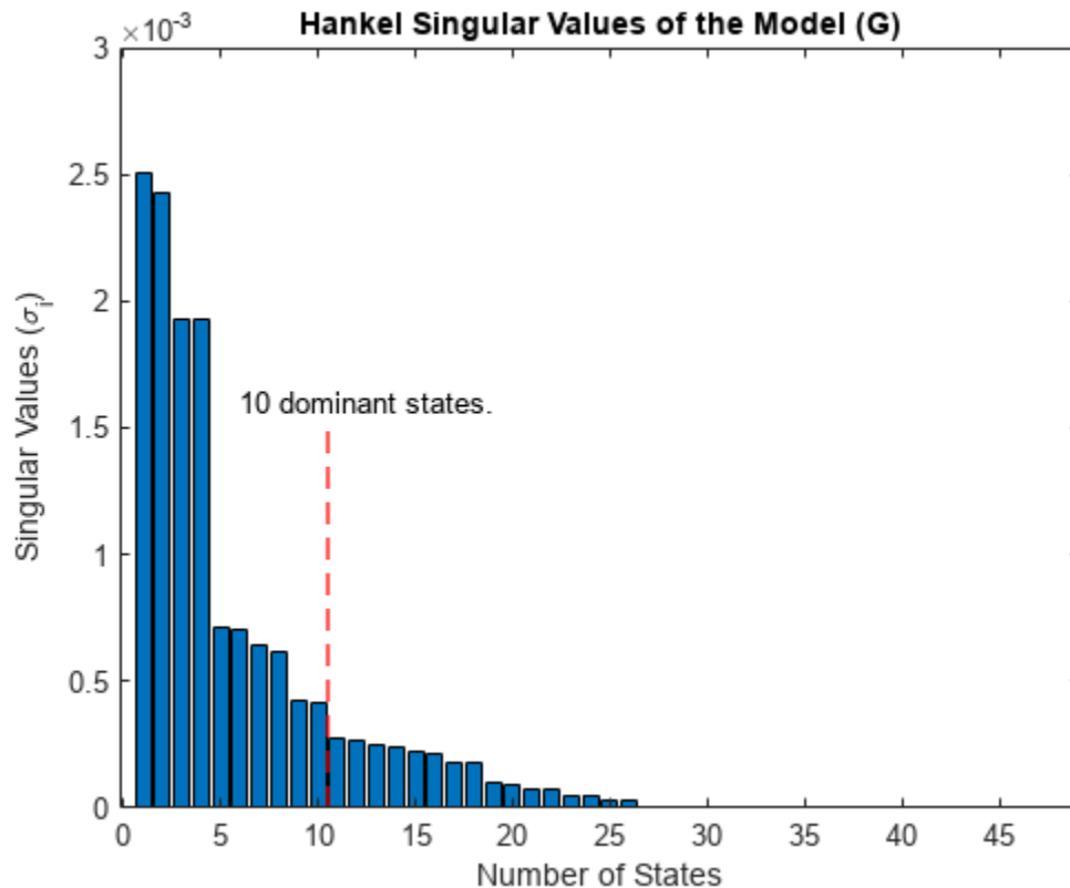
Figure 2: Hankel singular values of the model (G).
