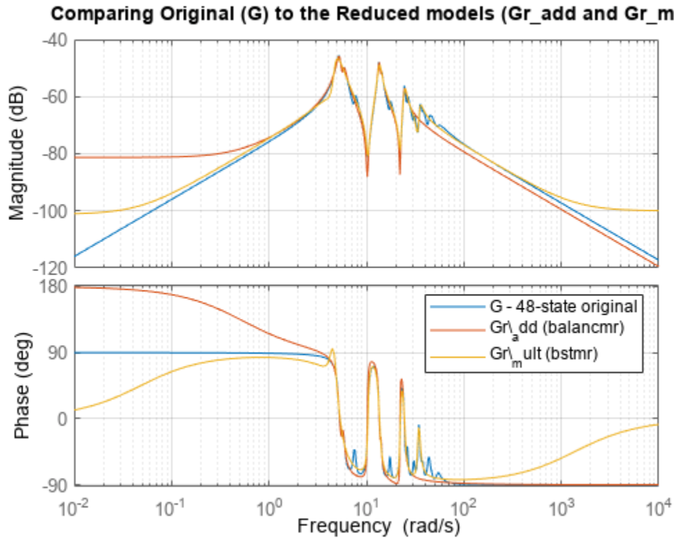
Figure 5: Comparing original (G) to the reduced models (Gr_add and Gr_mult)
