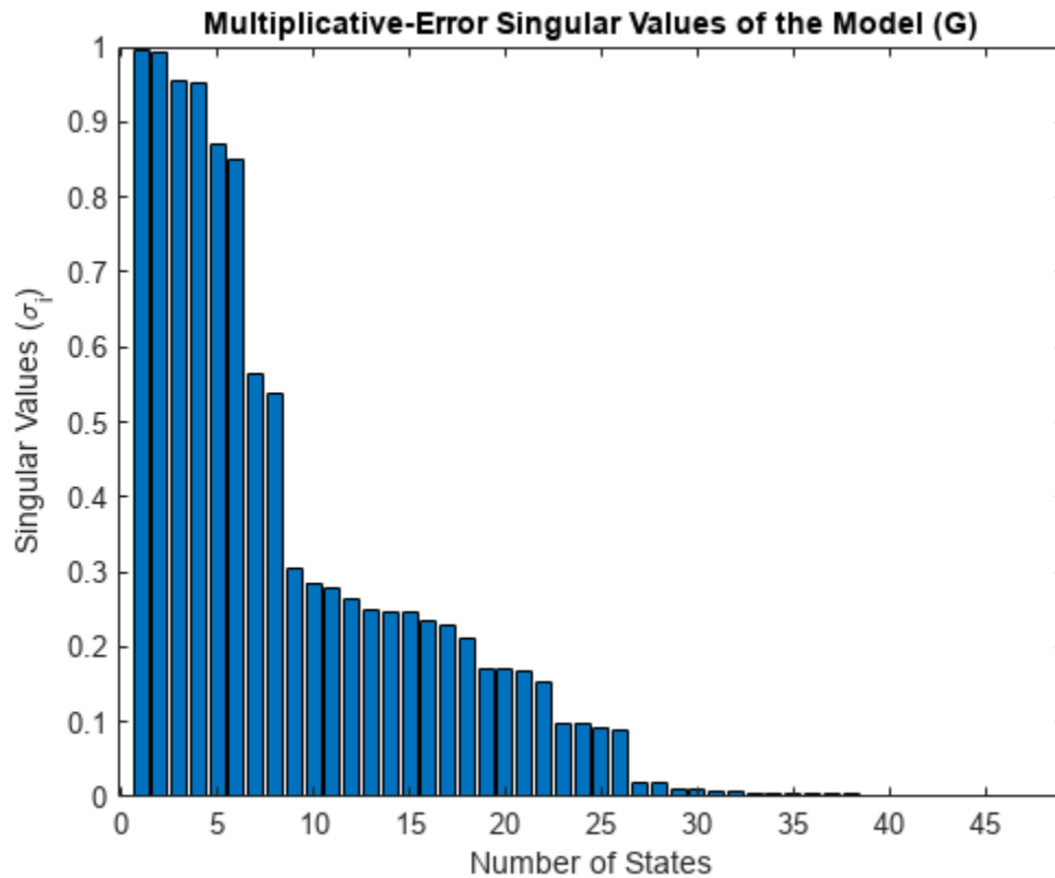
Figure 4: Multiplicative-error singular values of the model (G)
