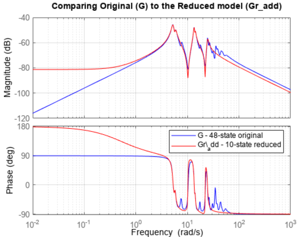
Figure 3: Comparing original (G) to the reduced model (Gr_add)
