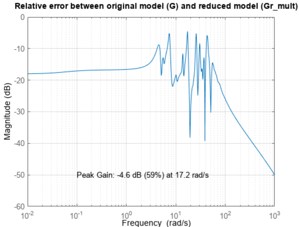
Figure 7: Relative error between original model ( G ) and reduced model ( G_{\text{reduced}} )
